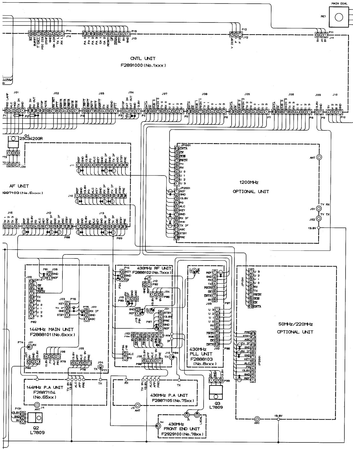
FT-736 CONNECTION DIAGRAM
